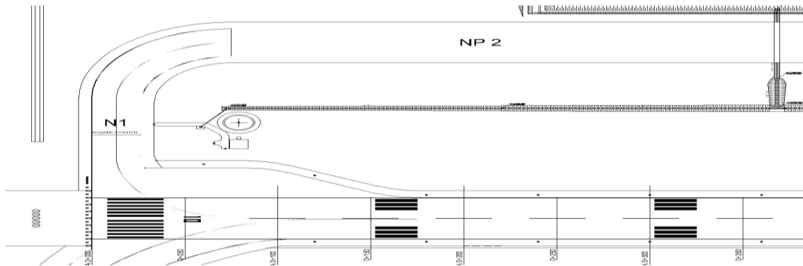
Gambar 4. Layout runway holding position N1 (posisi awal) Sumber : PT. Angkasa Pura I Cabang Bandara Juanda, 2013
